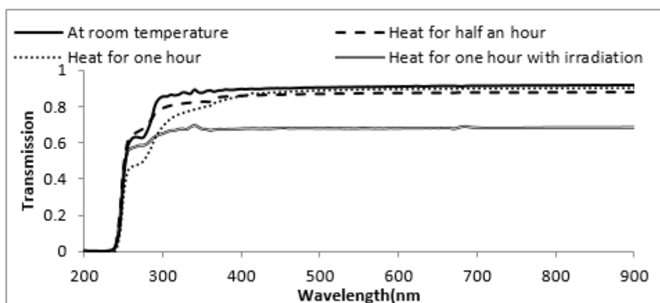
Figure 3. Transmission spectrum of PMMA thin films at annealing temperature and irradiation
